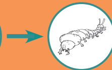
larva
