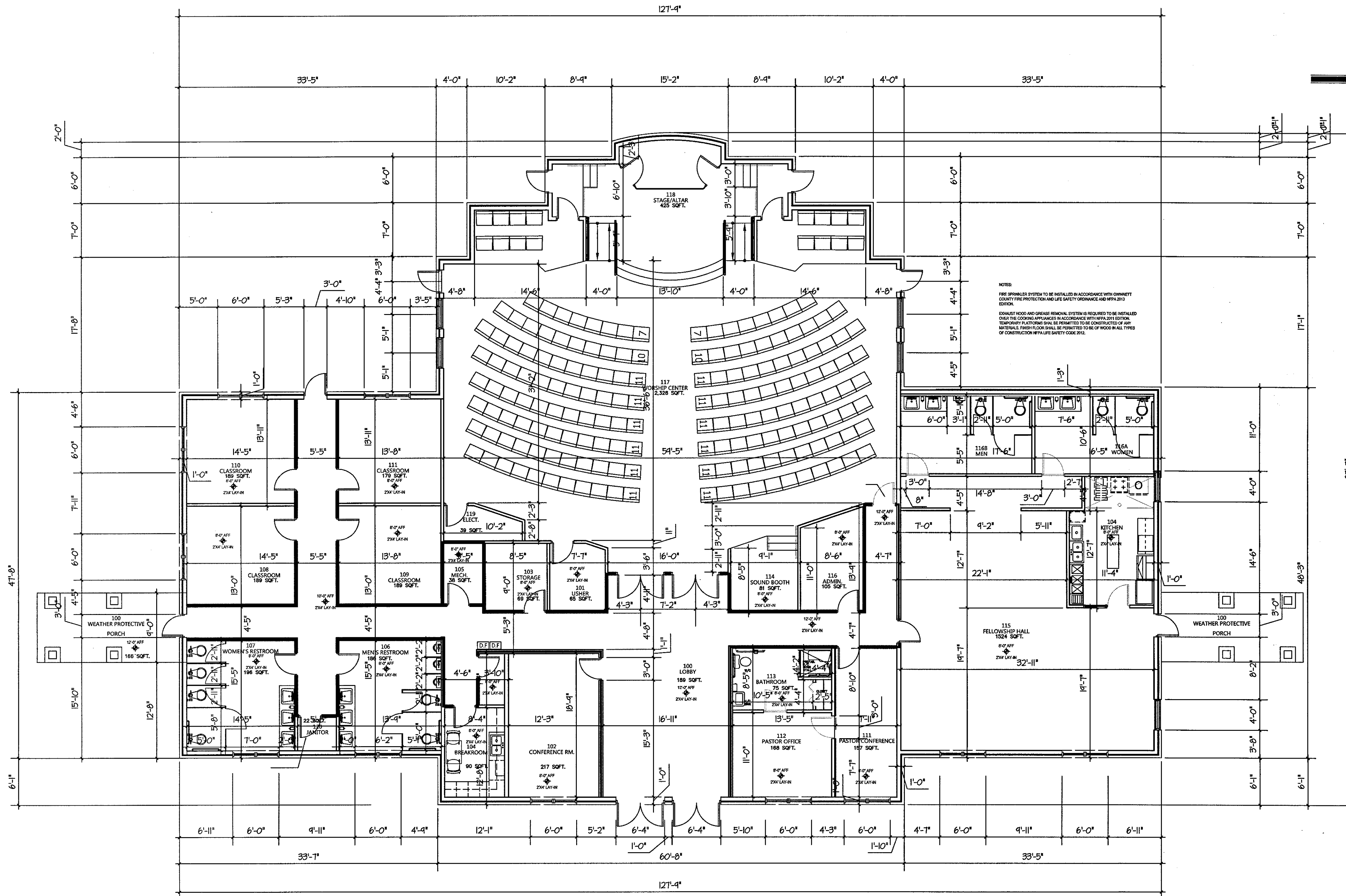
01 DIMENSIONED FLOOR PLAN AE-100 SCALE: 1/8" = 1' 0"
