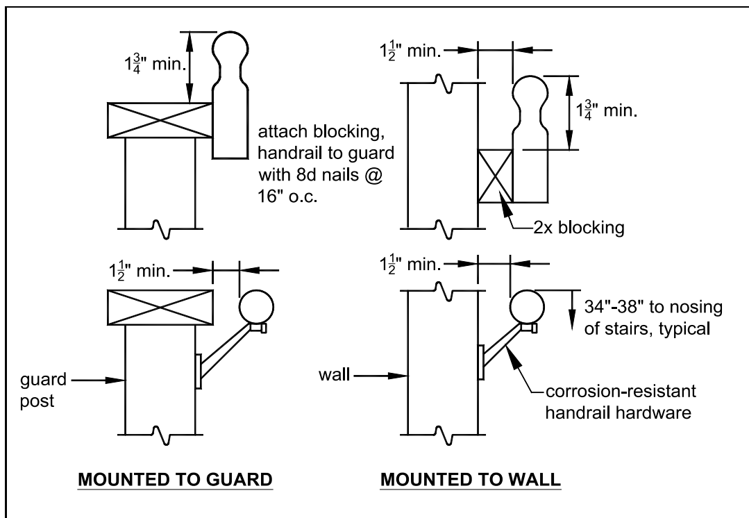
FIGURE 38: HANDRAIL REQUIREMENTS
