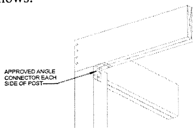
CORNER BEAM OVER POST
